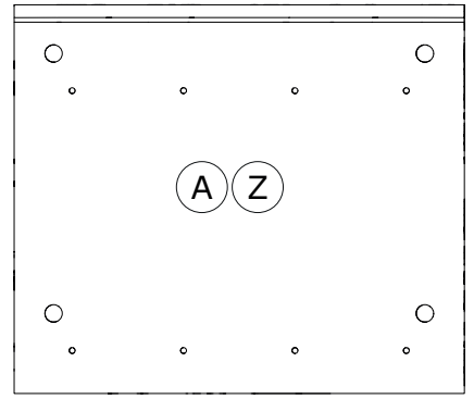
FI10327 388x335x16mm
