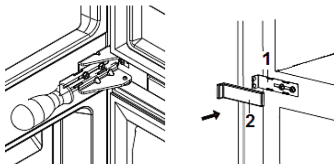
1: middle bracket; 2: middle bracket cover
