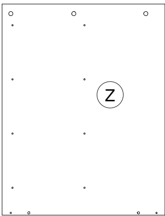
FI10334 748x583x16mm
